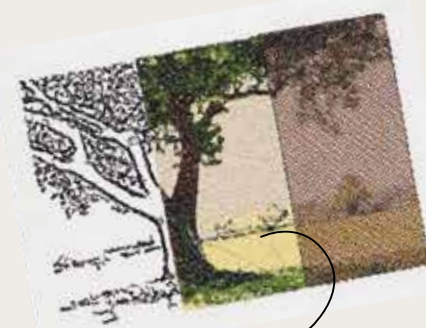
Convert Graphics
